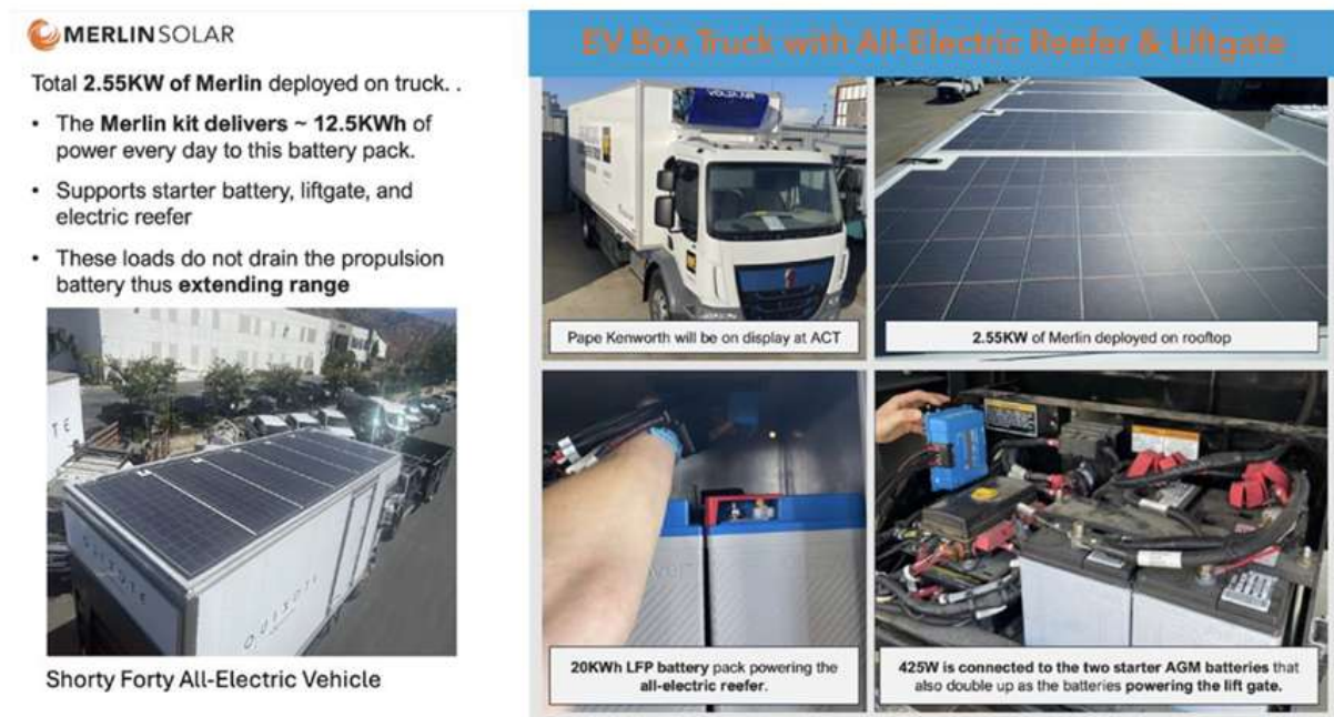
Figure 6.5. 2.55 kW Merlin Solar array integrated on the box truck roof, delivering daily solar energy to a 20 kWh LFP battery pack and AGM starter batteries to support refrigeration and liftgate loads independent of propulsion energy.
